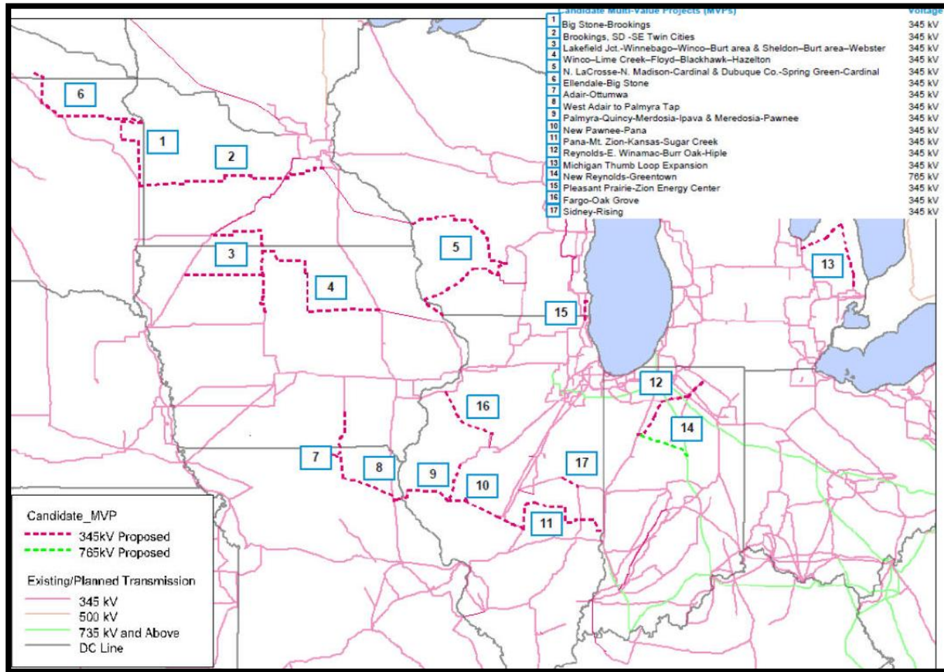
Figure RP-3: Candidate MVP Portfolio map for MTEP11 1
