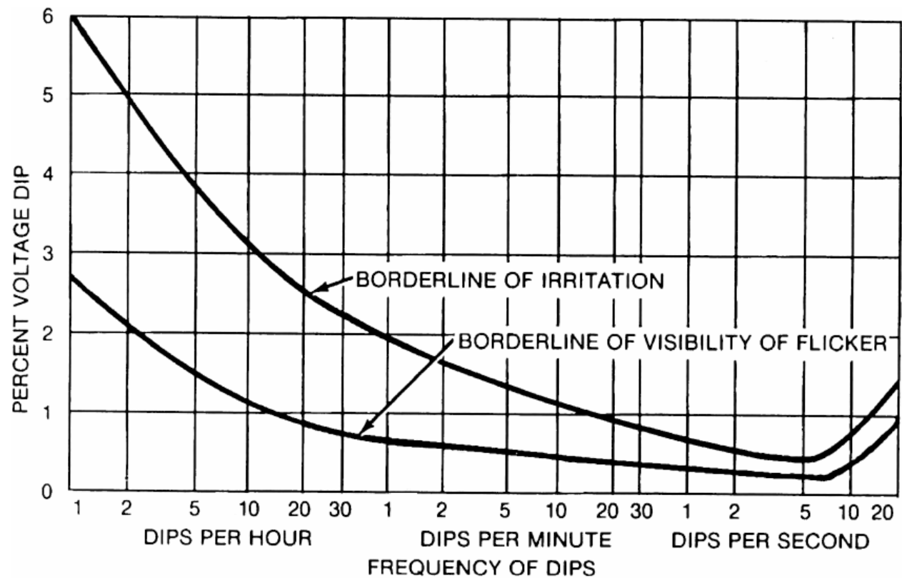
Figure 5-1: Flicker Tolerance Curve from IEEE Standard 1453
