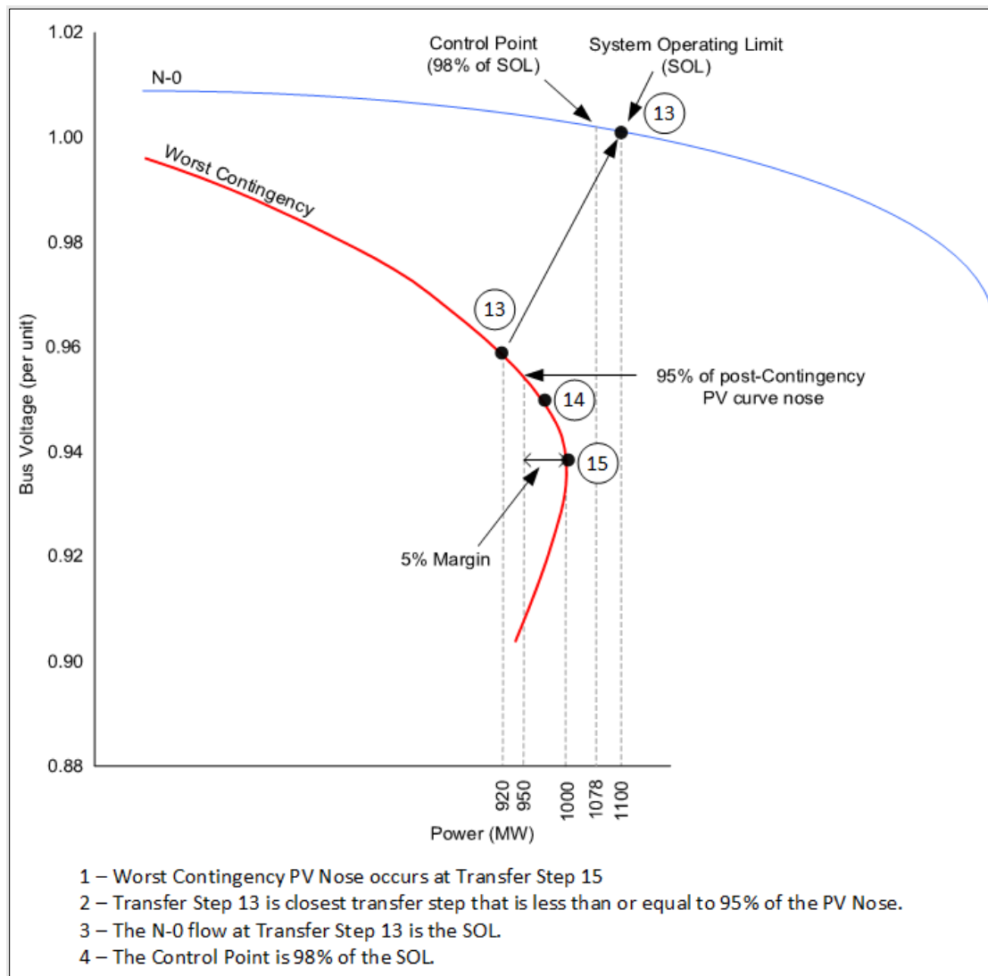
Figure 1.2-1: Practical Implementation of ATC Voltage Stability Criteria
