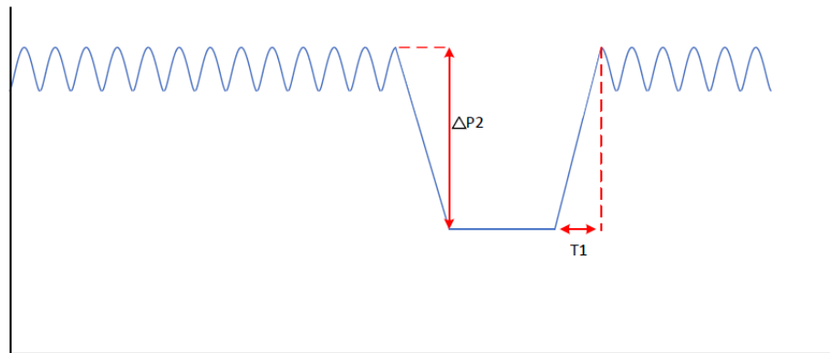
Figure 9.1-1: Active Power Criterion for \Delta P2 and T1, Example 1
