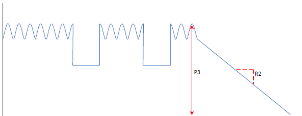
Figure 9.1-4: Active Power Criterion for P3 and R2 Example
