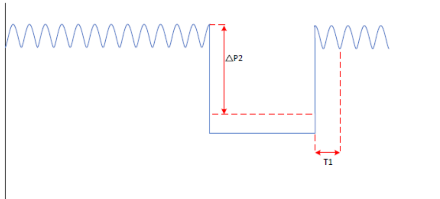
Figure 9.1-3: Active Power Criterion for \Delta P2 and T1 , Example 3
