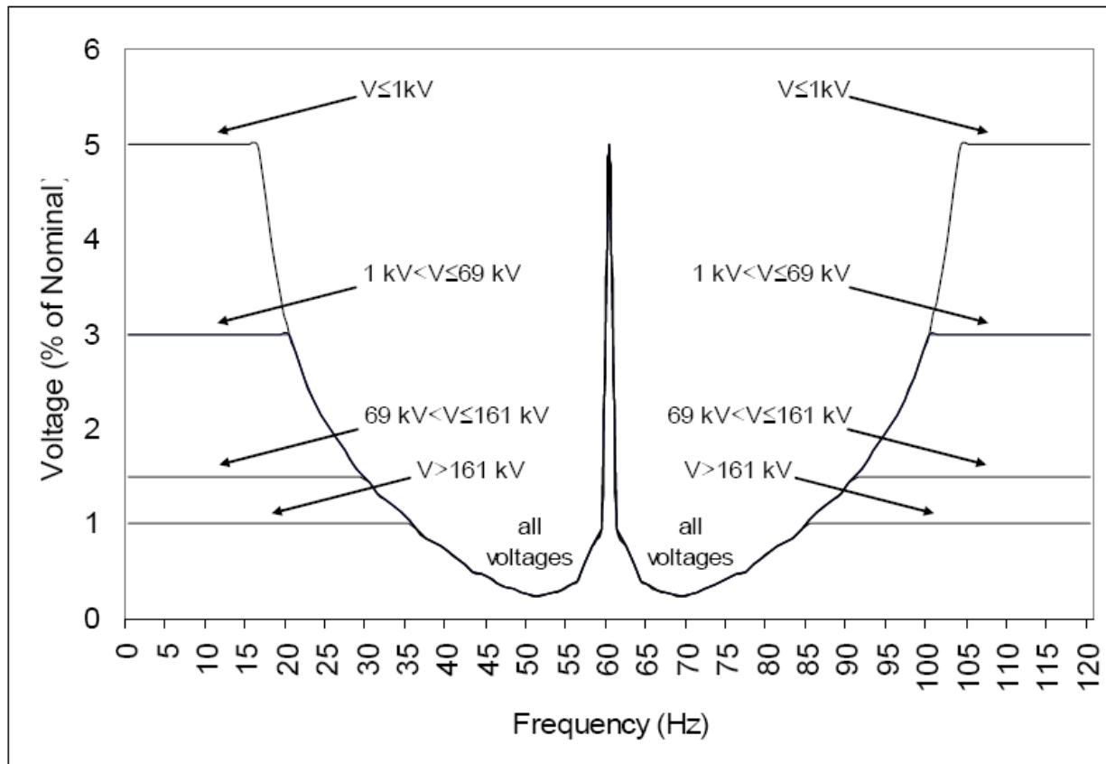
Figure 5-2: Flicker Limits Based on Interharmonic Voltages < 120 Hz (IEEE 1453)
